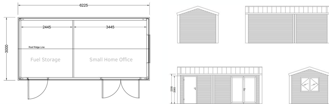
Sample plans and elevation of of multipurpose unit
